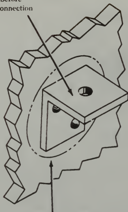
FIGURE 4-116. Bonding or grounding tab riveted to structure.
